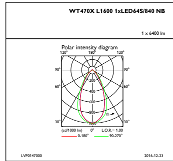
IFPC1_WT470XL16001xLED64S840NB
