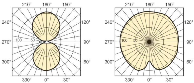
LDLD_SONHORTH_0001-Light distribution diagram
