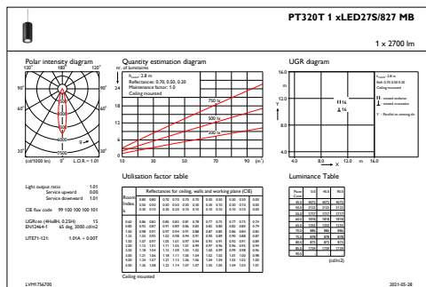
IFGU1_PT320T1xLED27S827MB
