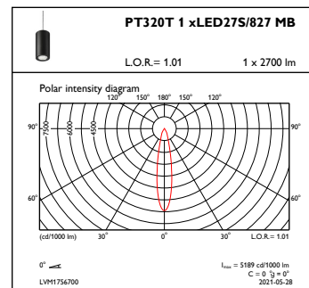
OFPC1_PT320T1xLED27S827MB
